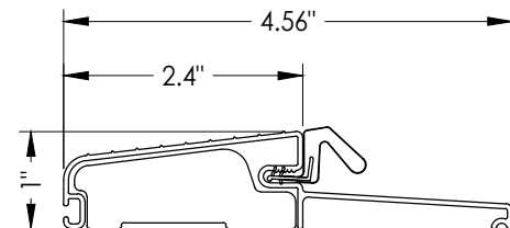
T12 OUTSWING THRESHOLD FOB4565
