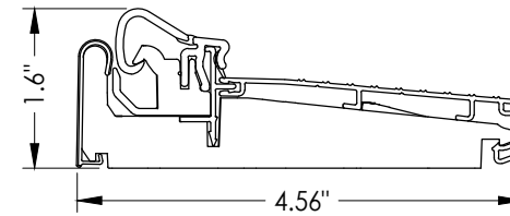
T8 INSWING ARTICULATING THRESHOLD ZAC4565RDS
