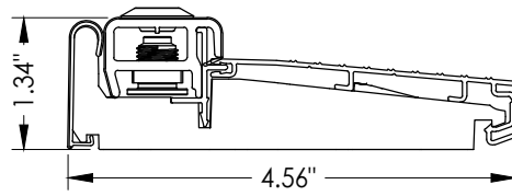
T4 INSWING ADJUSTABLE THRESHOLD ZAI4565RDS
