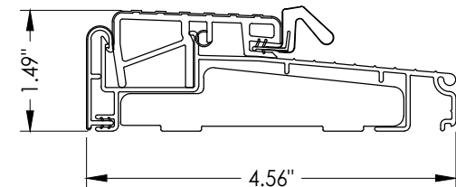
T9 OUTSWING THRESHOLD ZOBL4565
