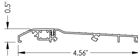
T13 INSWING/OUTSWING ACCESSIBLE THRESHOLD ADAPI4562 / ADAPO4562
