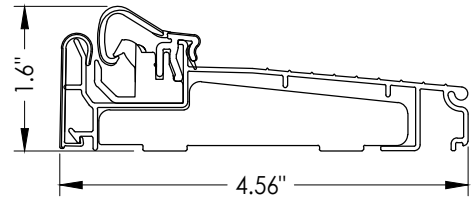
T5 INSWING ARTICULATING THRESHOLD ZACL4565
