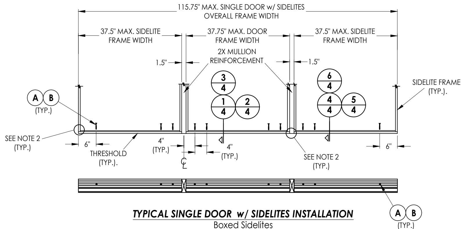
TYPICAL SINGLE DOOR w/ SIDELITES INSTALLATION Continuous Head & Sill
