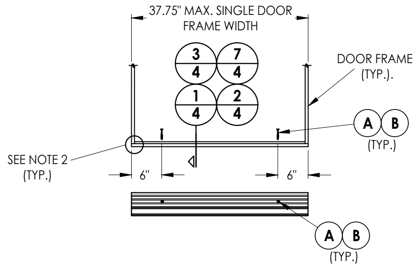
TYPICAL SINGLE DOOR INSTALLATION
