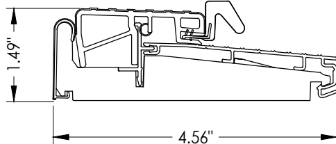
T11 OUTSWING THRESHOLD ZOB4565RDS
