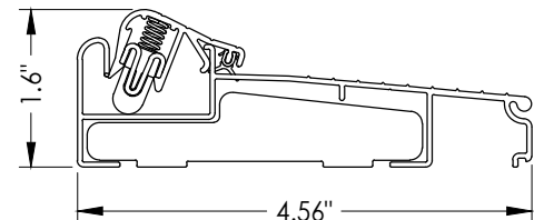
T6 INSWING ARTICULATING THRESHOLD ZACLAA4565
