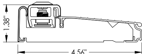
T3 INSWING ADJUSTABLE THRESHOLD ZAI4565FN
