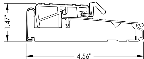
T10 OUTSWING THRESHOLD ZOB4565FN
